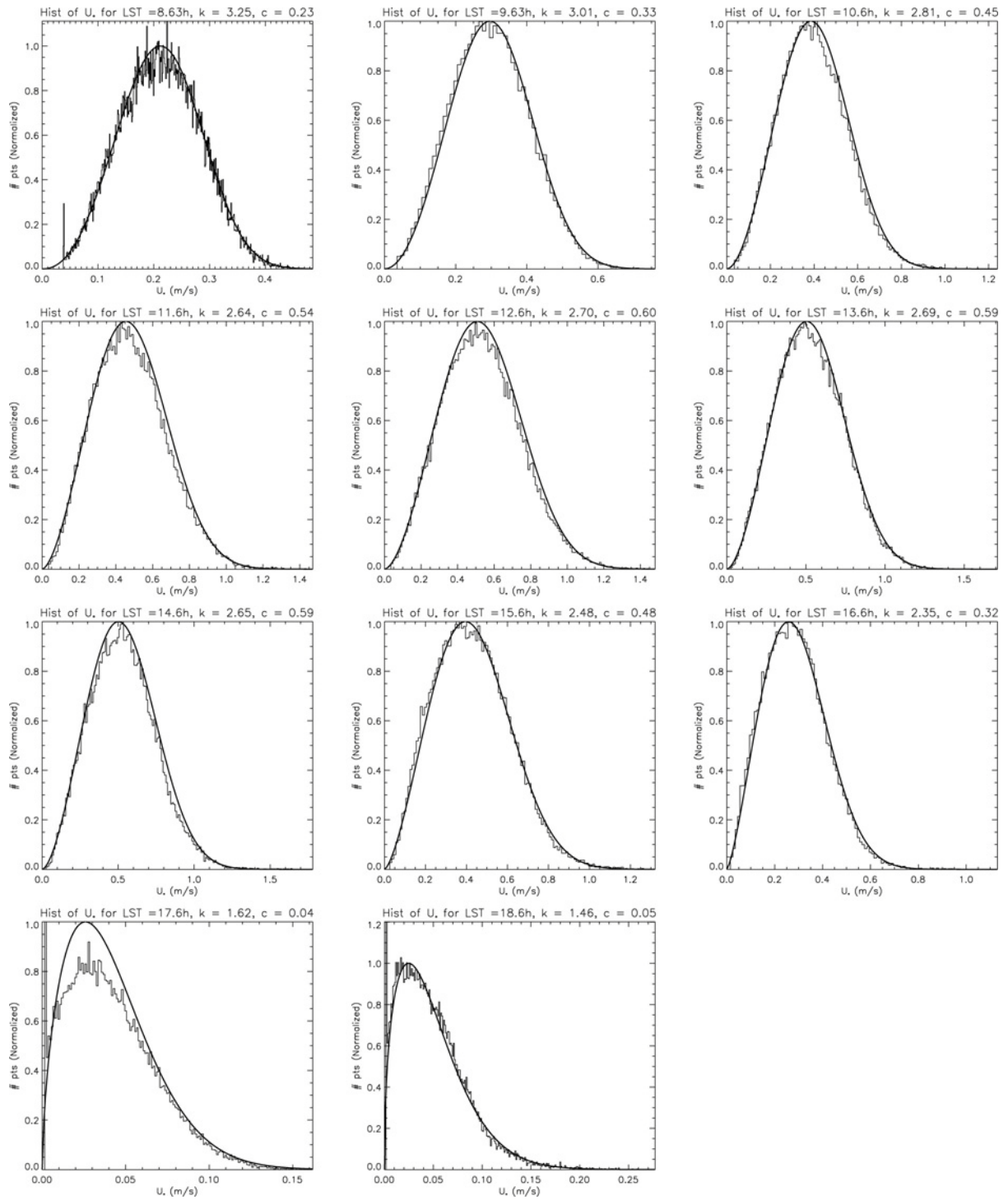
Supplemental Figure 1. Weibull curves fit to LES friction velocities, from the Viking Lander 1 site simulation at L_s=120^\circ and with Case 1 initial winds. ( suppfigure1.jpg ) ( suppfigure1.txt ).
