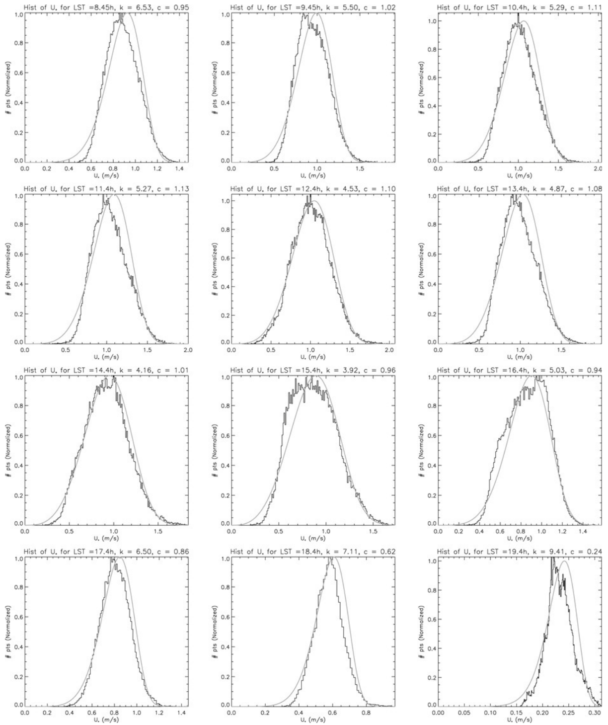
Supplemental Figure 2. Weibull curves fit to LES friction velocities, from the Phoenix landing site simulation at L_s=120^\circ and with Case 3 “strong winds with wind shear” initial winds ( suppfigure2.jpg ) ( suppfigure2.txt ).
